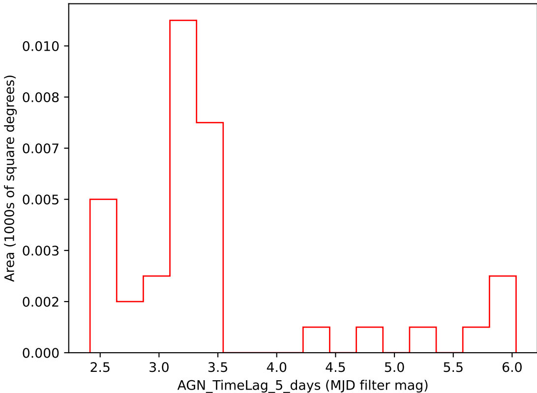
scp_reweight_v3.3_10yrs i band: AGN_TimeLag_5_days
