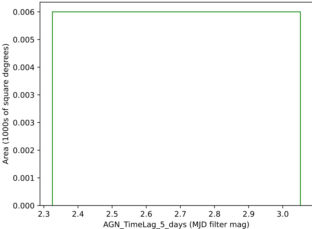
scp_reweight_v3.3_10yrs g band: AGN_TimeLag_5_days
