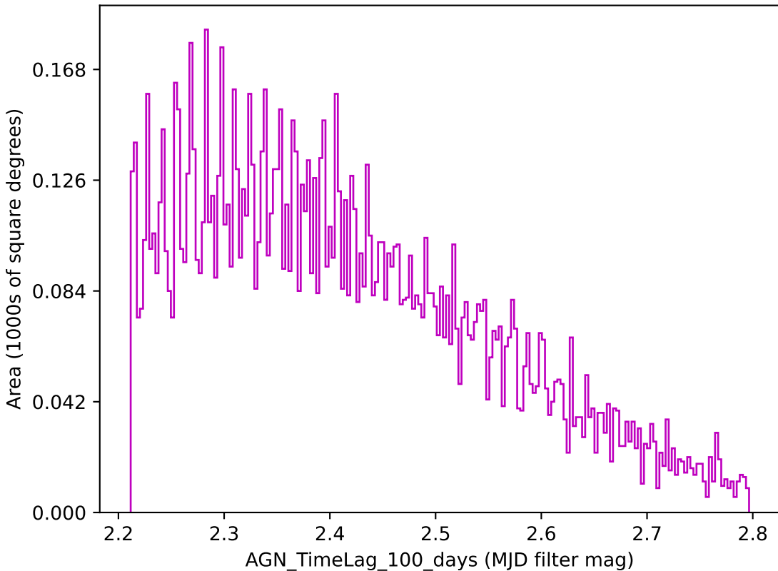
scp_reweight_v3.3_10yrs z band: AGN_TimeLag_100_days
