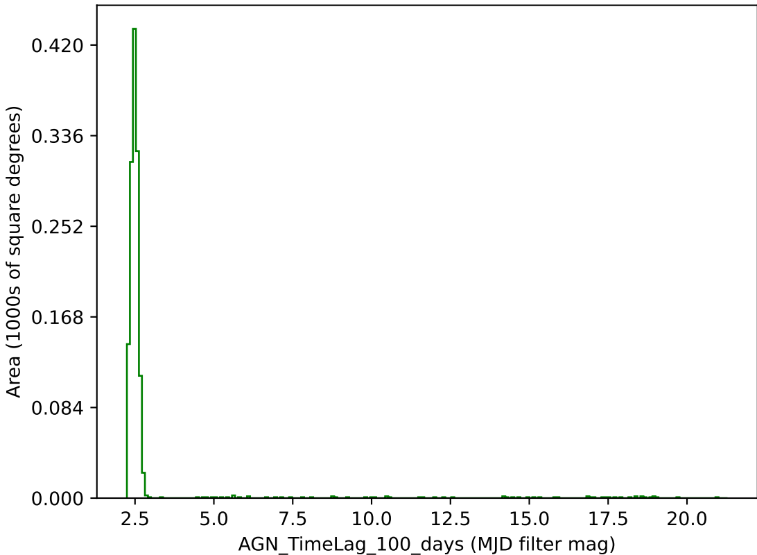
scp_reweight_v3.3_10yrs g band: AGN_TimeLag_100_days
