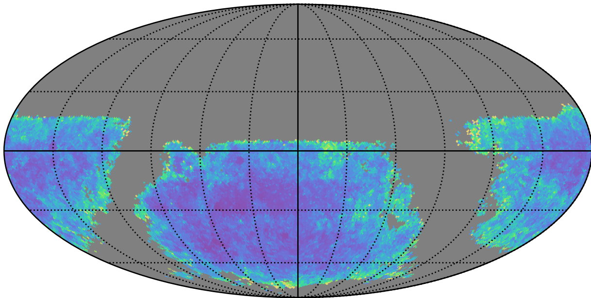
scp_reweight_v3.3_10yrs u band: AGN SF_uncert
