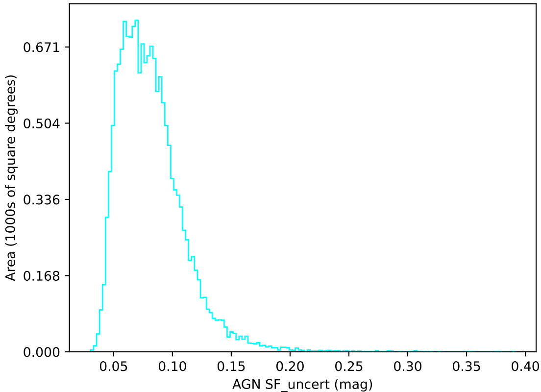
scp_reweight_v3.3_10yrs u band: AGN SF_uncert
