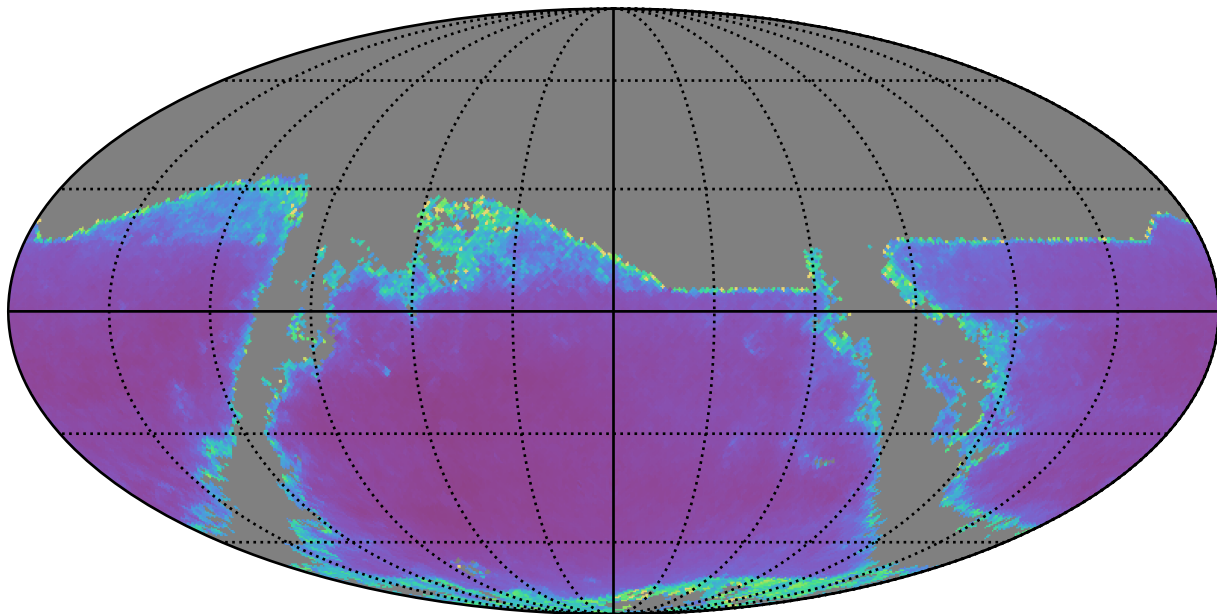
scp_reweight_v3.3_10yrs r band: AGN SF_uncert
