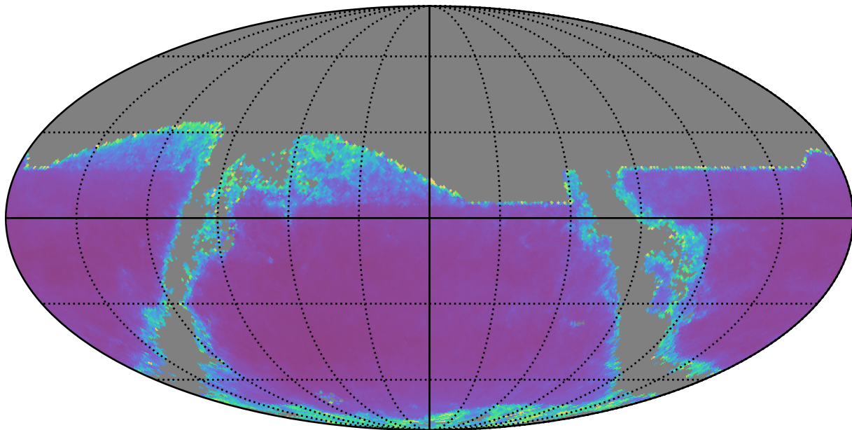
scp_reweight_v3.3_10yrs i band: AGN SF_uncert
