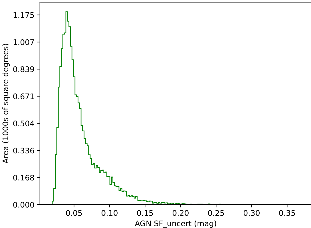
scp_reweight_v3.3_10yrs g band: AGN SF_uncert
