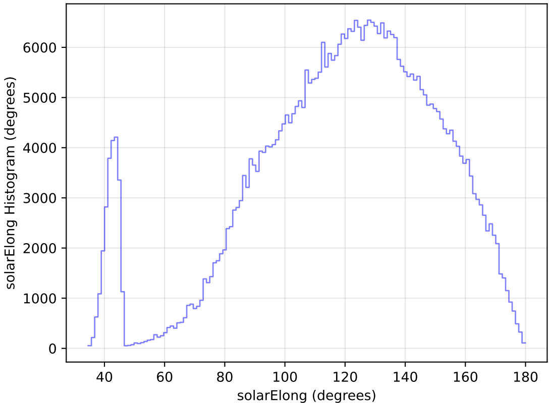
scp_reweight_v3.3_10yrs WFD z band: solarElong Histogram
