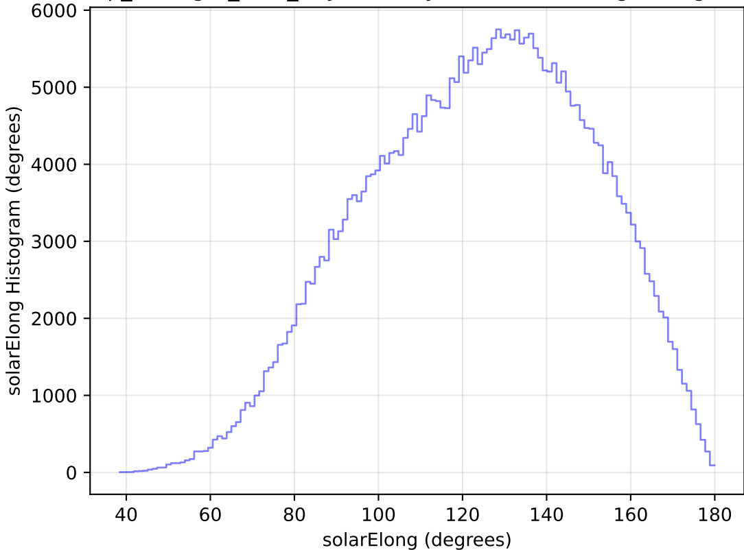
scp_reweight_v3.3_10yrs WFD y band: solarElong Histogram
