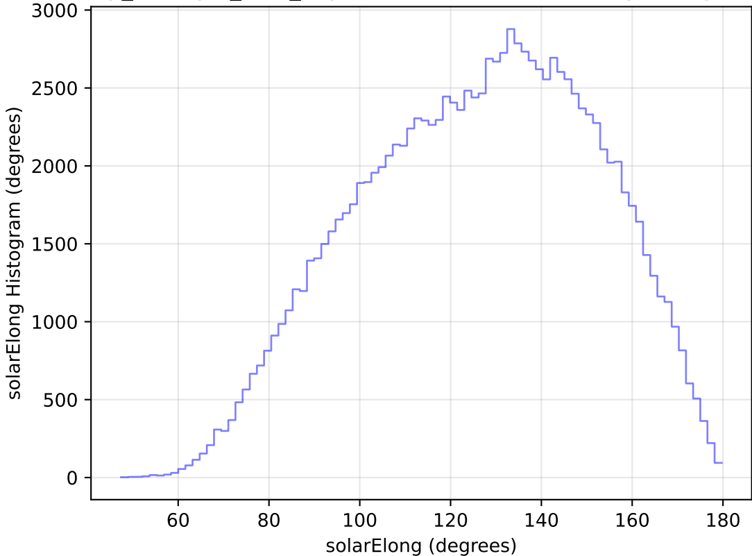
scp_reweight_v3.3_10yrs WFD u band: solarElong Histogram
