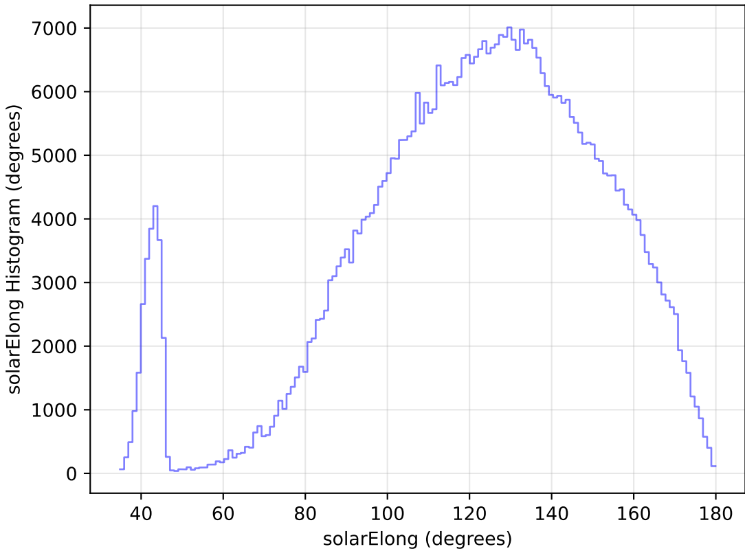
scp_reweight_v3.3_10yrs WFD i band: solarElong Histogram
