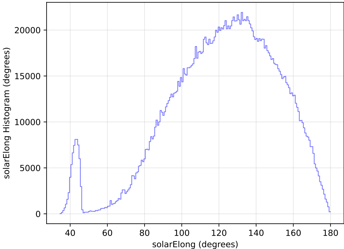
scp_reweight_v3.3_10yrs WFD all bands: solarElong Histogram
