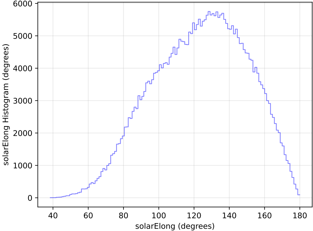
scp_reweight_v3.3_10yrs All sky y band: solarElong Histogram
