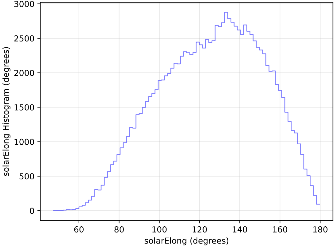
scp_reweight_v3.3_10yrs All sky u band: solarElong Histogram
