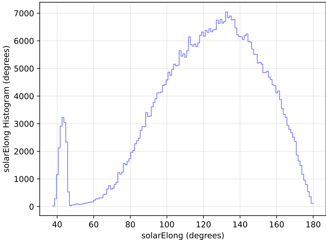
scp_reweight_v3.3_10yrs All sky r band: solarElong Histogram
