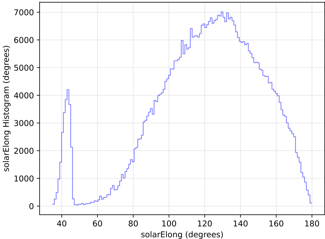
scp_reweight_v3.3_10yrs All sky i band: solarElong Histogram
