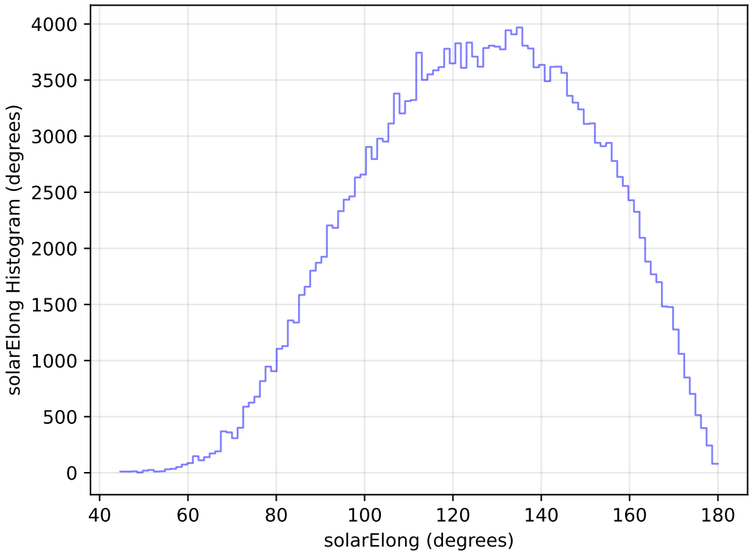
scp_reweight_v3.3_10yrs All sky g band: solarElong Histogram
