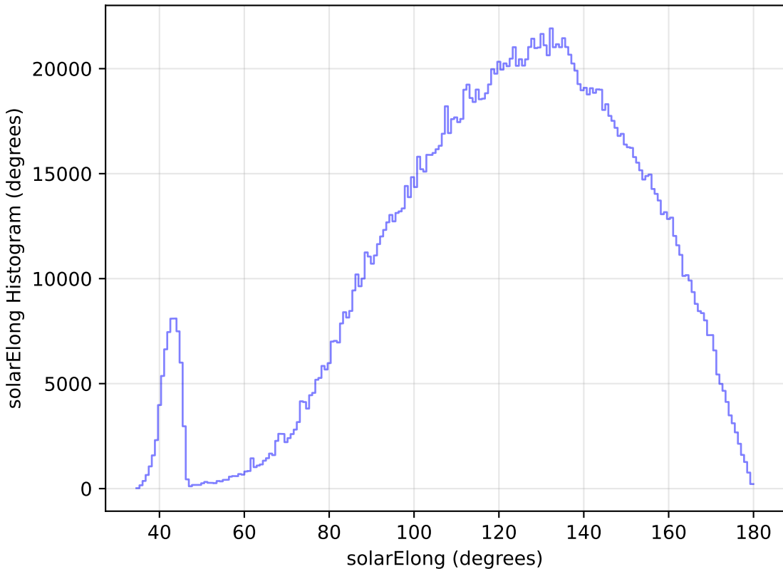
scp_reweight_v3.3_10yrs All sky all bands: solarElong Histogram
