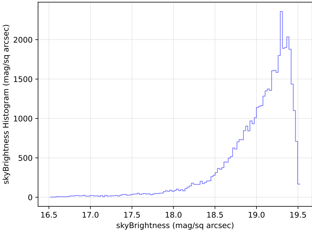
scp_reweight_v3.3_10yrs Yr 1 z band: skyBrightness Histogram
