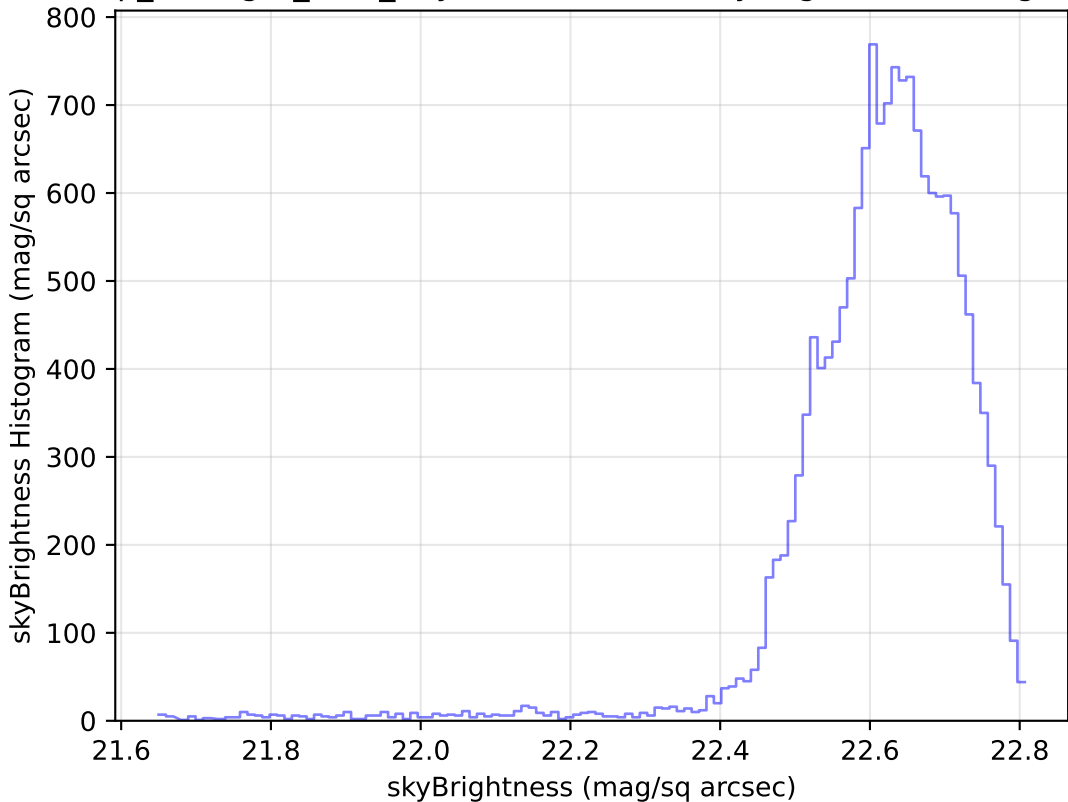
scp_reweight_v3.3_10yrs Yr 1 u band: skyBrightness Histogram
