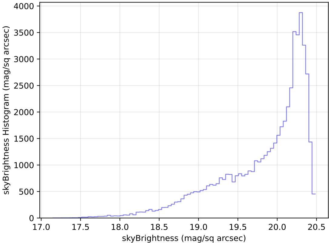
scp_reweight_v3.3_10yrs Yr 1 i band: skyBrightness Histogram
