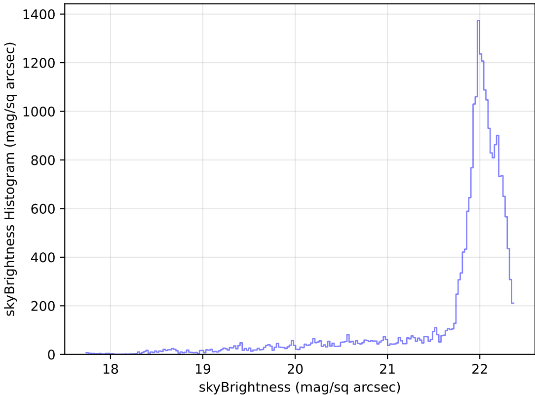
scp_reweight_v3.3_10yrs Yr 1 g band: skyBrightness Histogram
