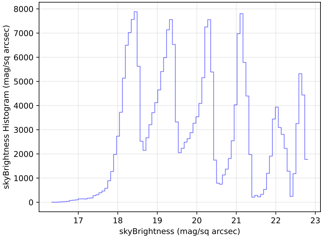
scp_reweight_v3.3_10yrs Yr 1 all bands: skyBrightness Histogram
