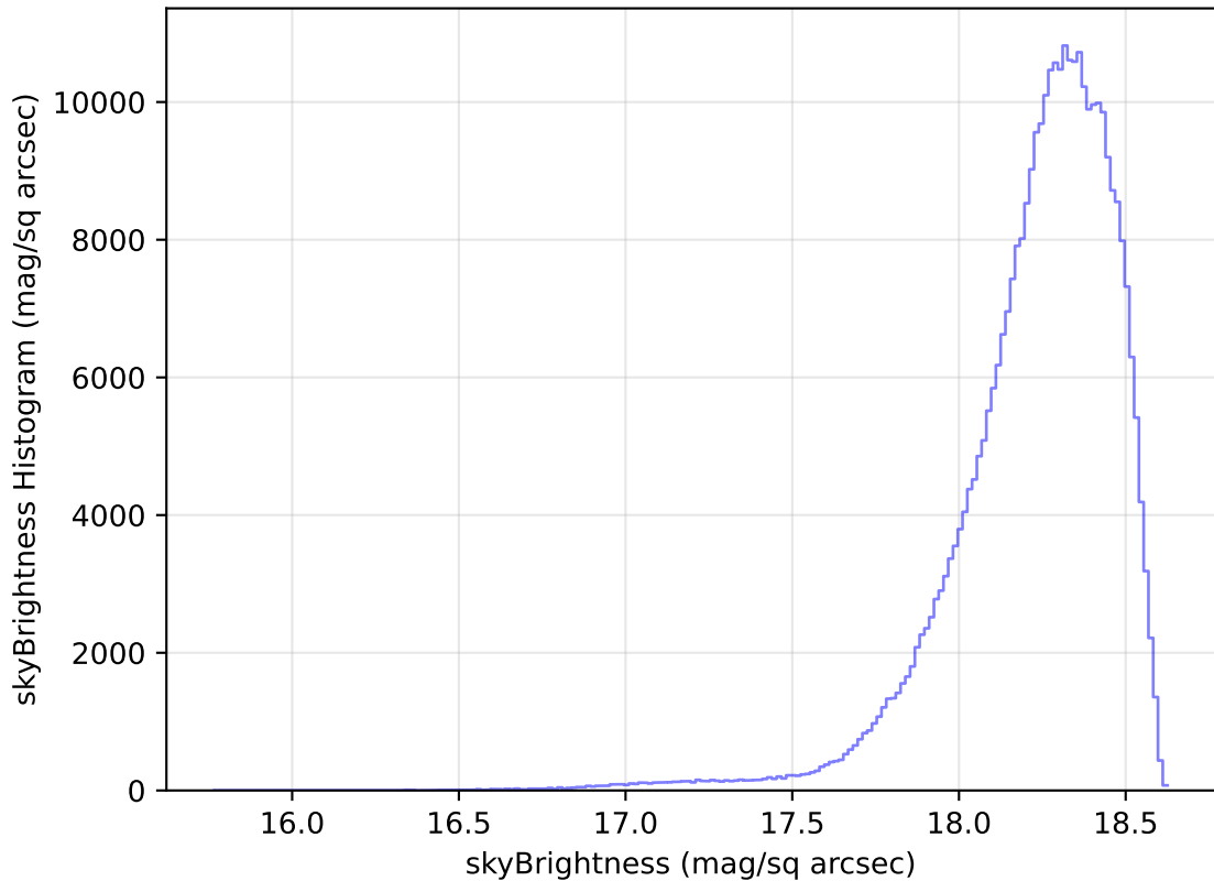
scp_reweight_v3.3_10yrs WFD y band: skyBrightness Histogram
