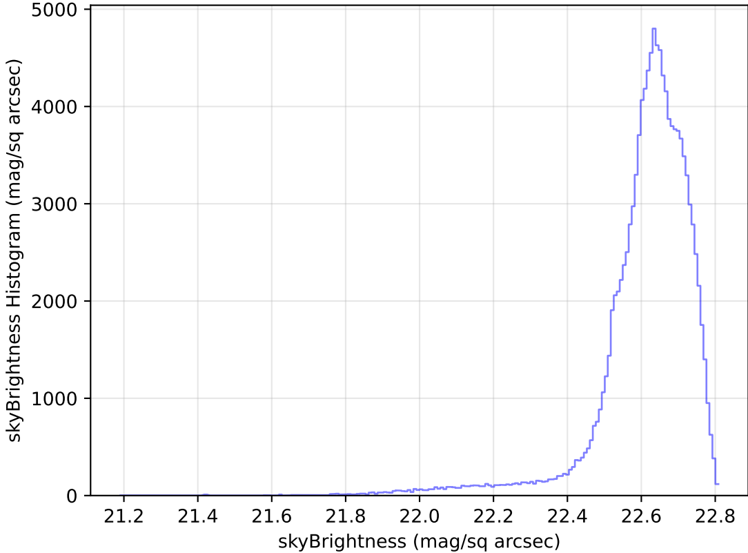
scp_reweight_v3.3_10yrs WFD u band: skyBrightness Histogram
