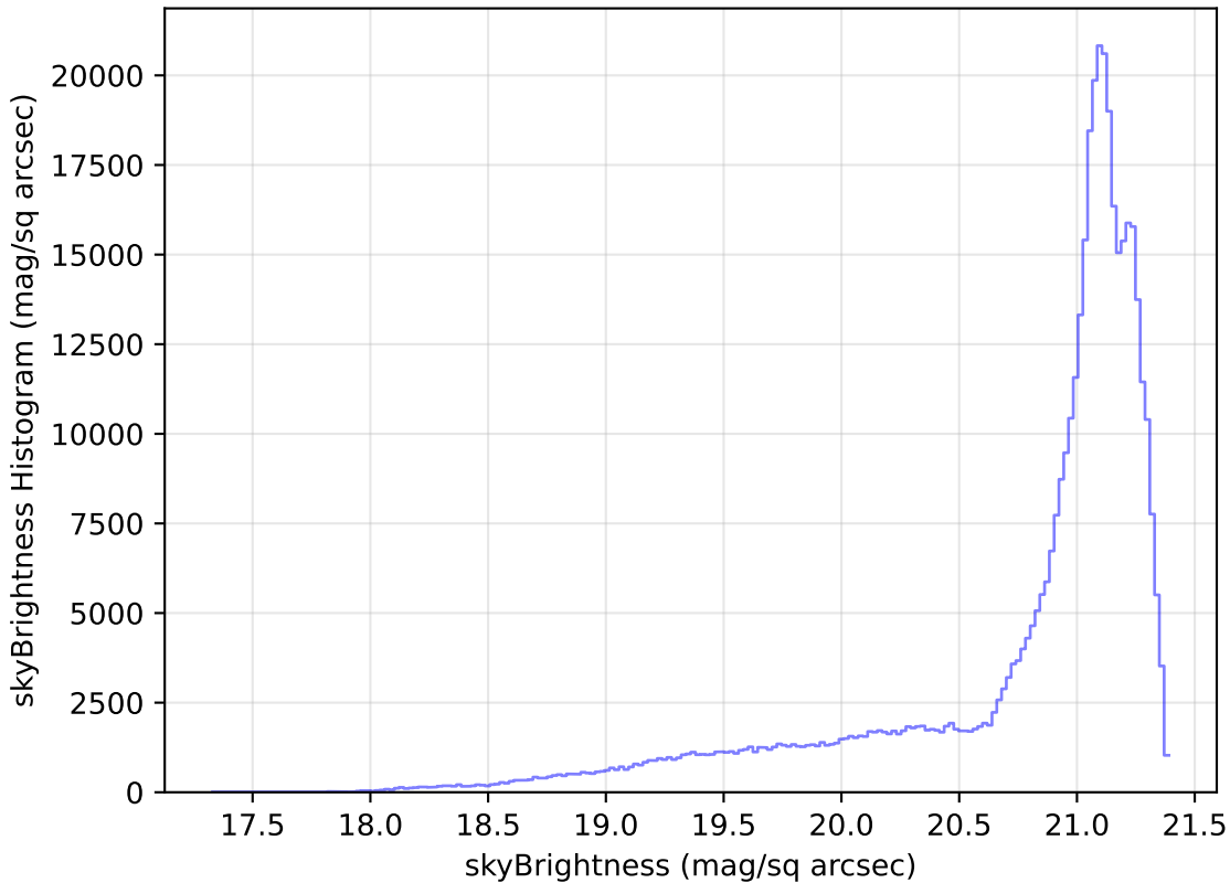
scp_reweight_v3.3_10yrs WFD r band: skyBrightness Histogram
