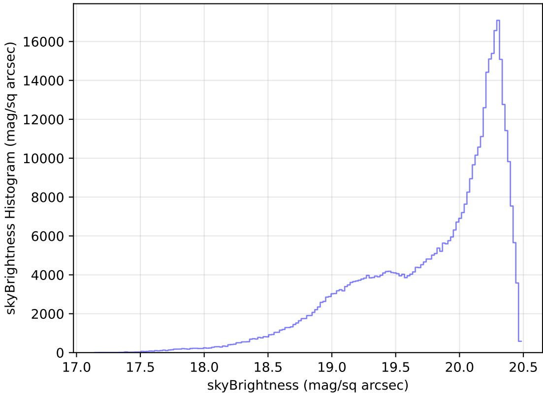
scp_reweight_v3.3_10yrs WFD i band: skyBrightness Histogram
