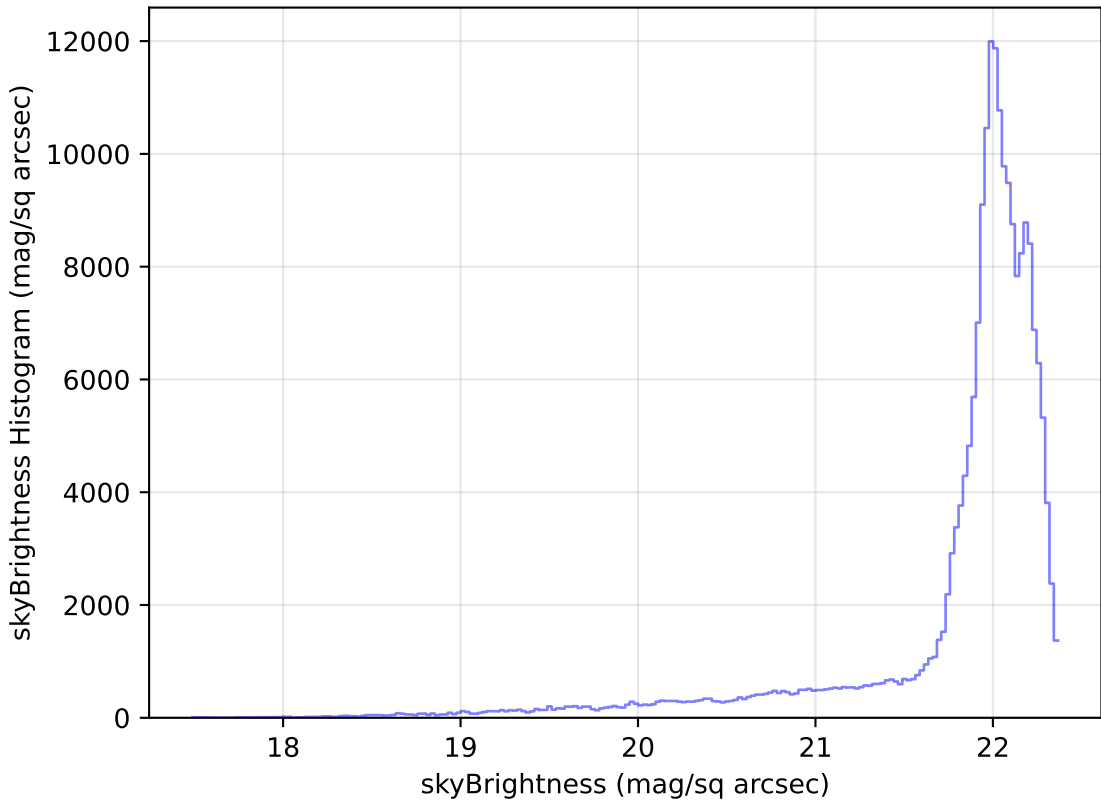
scp_reweight_v3.3_10yrs WFD g band: skyBrightness Histogram
