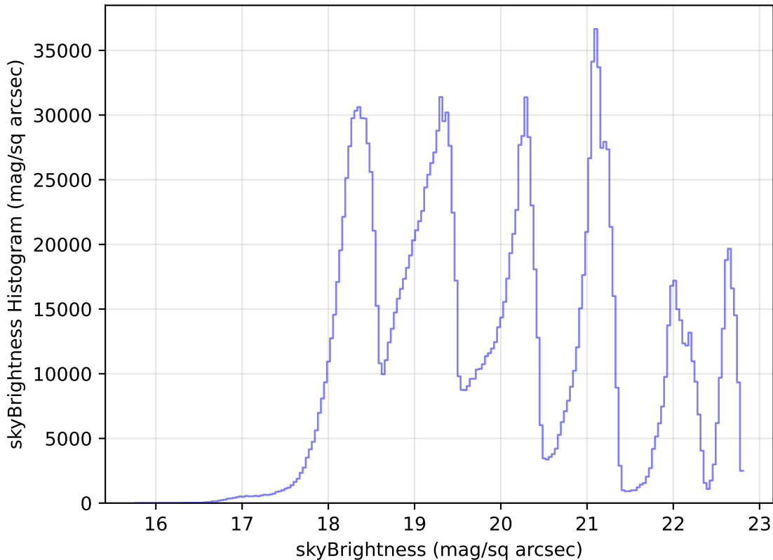
scp_reweight_v3.3_10yrs WFD all bands: skyBrightness Histogram
