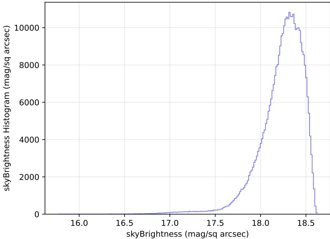
scp_reweight_v3.3_10yrs All sky y band: skyBrightness Histogram
