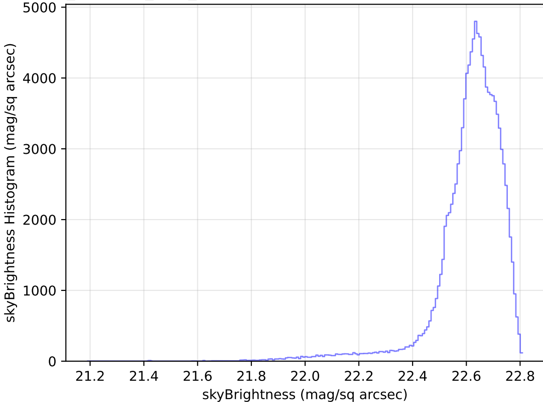
scp_reweight_v3.3_10yrs All sky u band: skyBrightness Histogram
