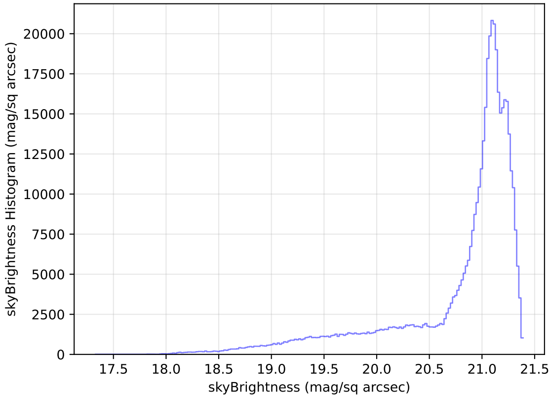
scp_reweight_v3.3_10yrs All sky r band: skyBrightness Histogram
