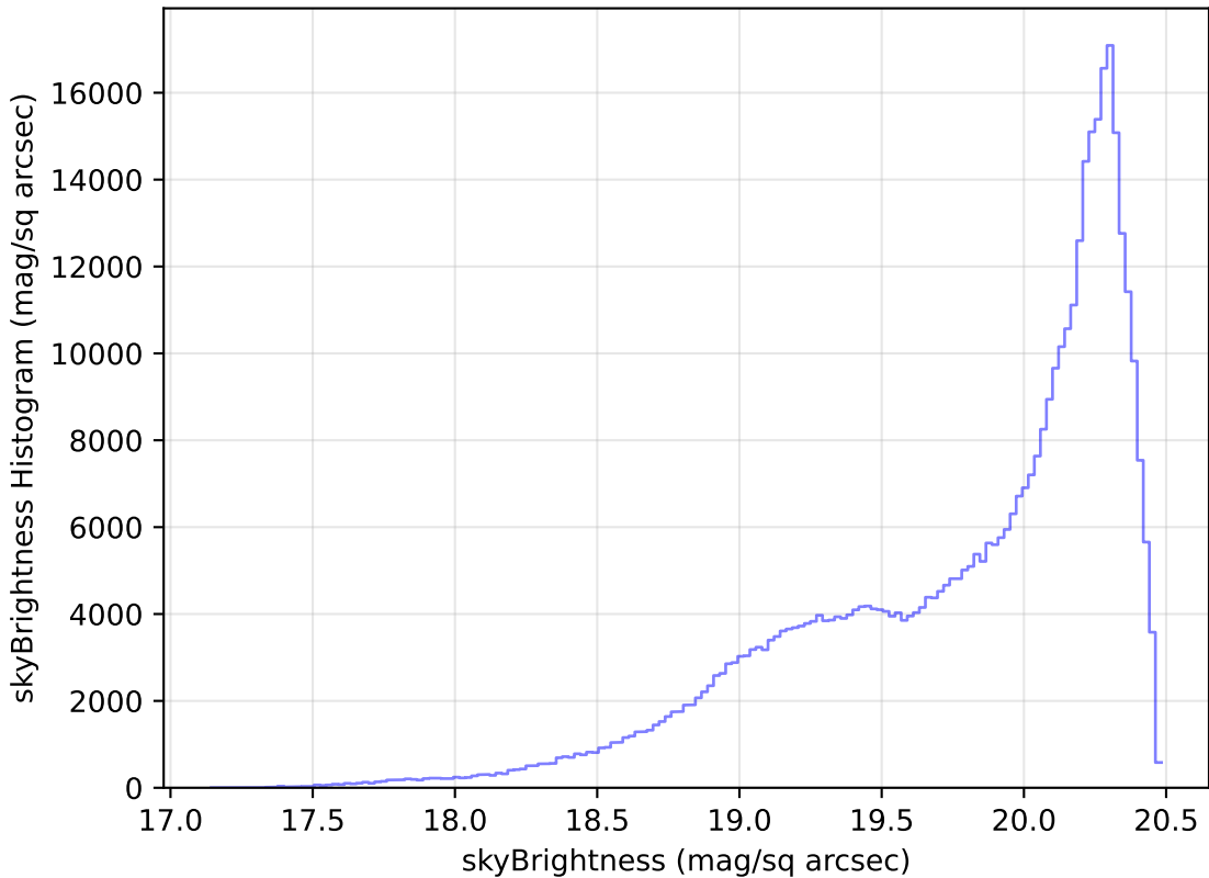
scp_reweight_v3.3_10yrs All sky i band: skyBrightness Histogram
