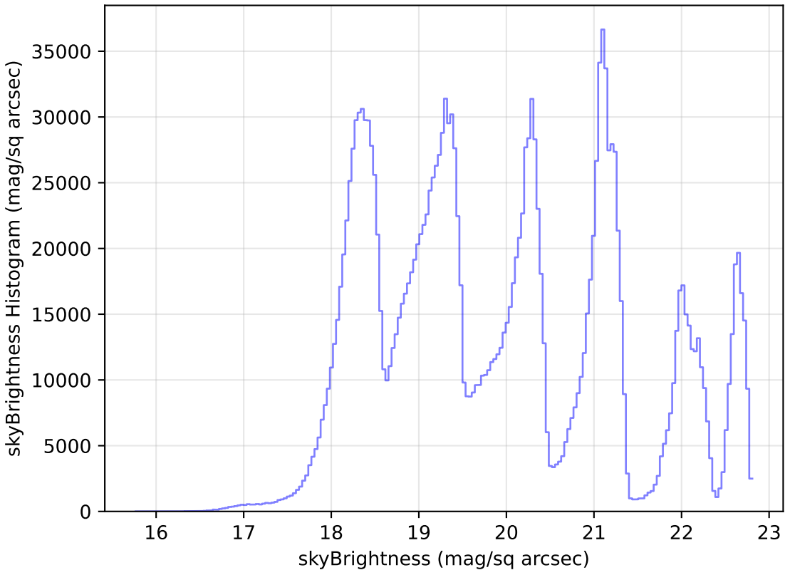
scp_reweight_v3.3_10yrs All sky all bands: skyBrightness Histogram
