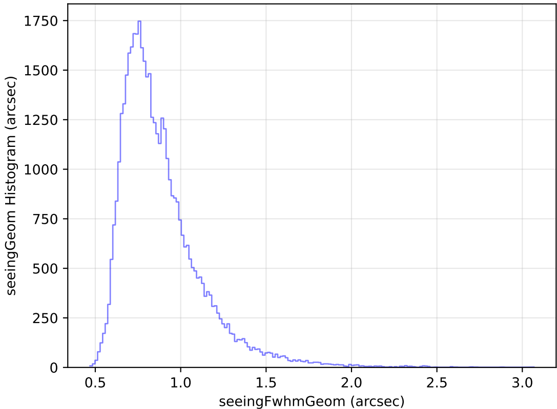
scp_reweight_v3.3_10yrs Yr 1 z band: seeingGeom Histogram
