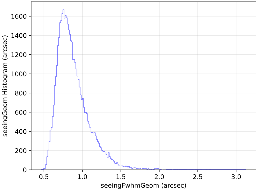
scp_reweight_v3.3_10yrs Yr 1 y band: seeingGeom Histogram
