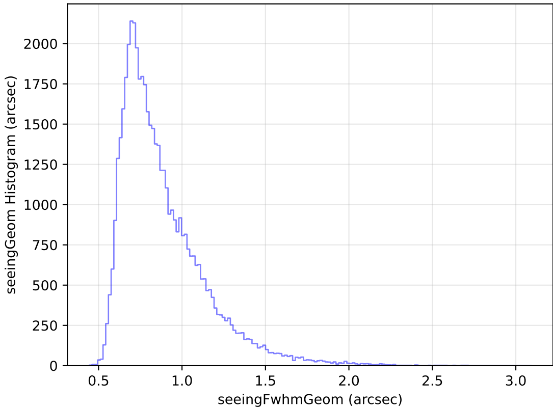
scp_reweight_v3.3_10yrs Yr 1 r band: seeingGeom Histogram
