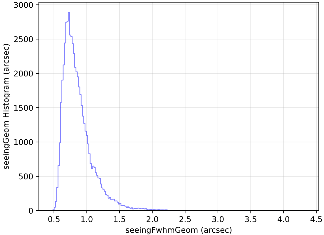
scp_reweight_v3.3_10yrs Yr 1 i band: seeingGeom Histogram
