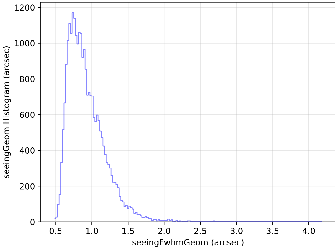
scp_reweight_v3.3_10yrs Yr 1 g band: seeingGeom Histogram
