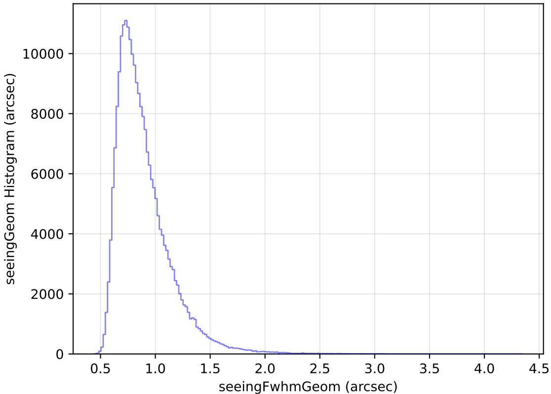
scp_reweight_v3.3_10yrs Yr 1 all bands: seeingGeom Histogram
