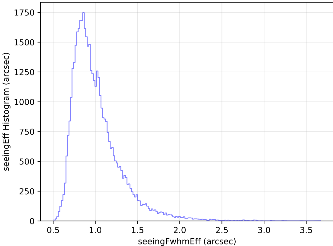
scp_reweight_v3.3_10yrs Yr 1 z band: seeingEff Histogram
