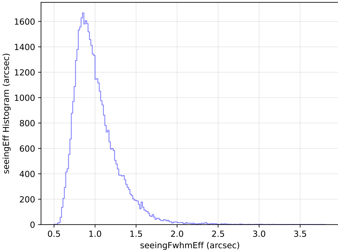
scp_reweight_v3.3_10yrs Yr 1 y band: seeingEff Histogram
