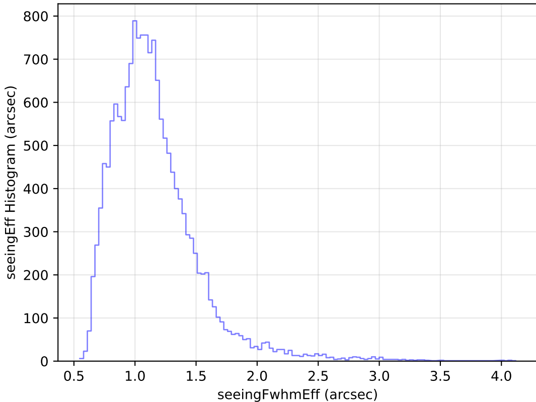
scp_reweight_v3.3_10yrs Yr 1 u band: seeingEff Histogram
