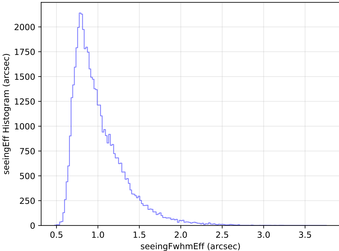
scp_reweight_v3.3_10yrs Yr 1 r band: seeingEff Histogram
