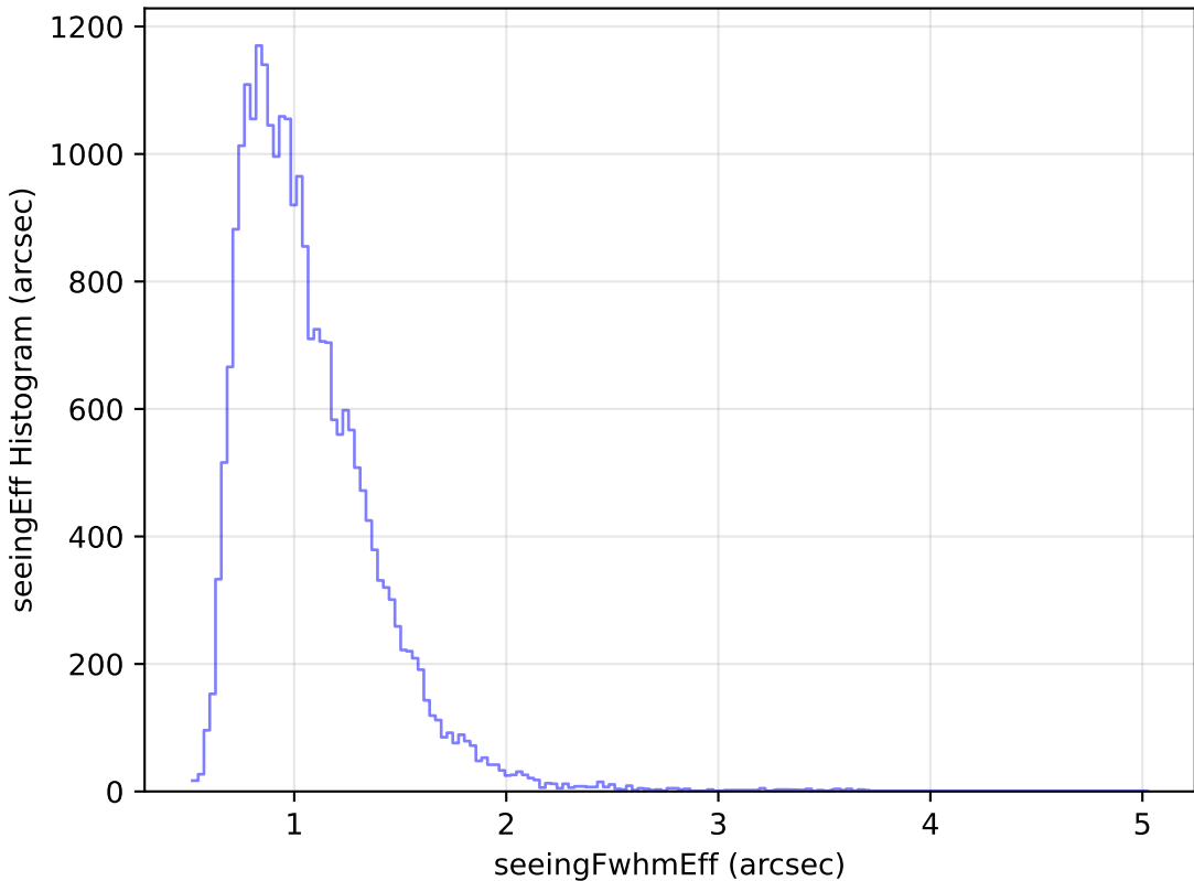
scp_reweight_v3.3_10yrs Yr 1 g band: seeingEff Histogram
