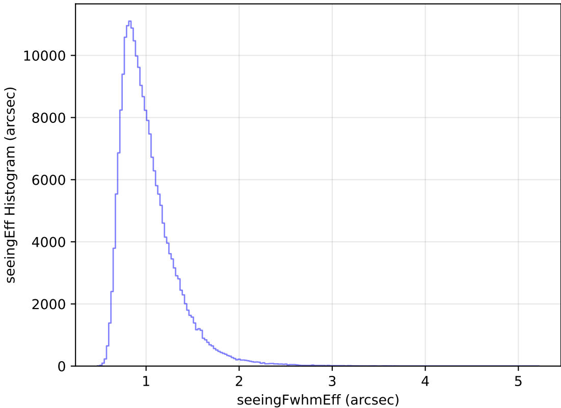
scp_reweight_v3.3_10yrs Yr 1 all bands: seeingEff Histogram
