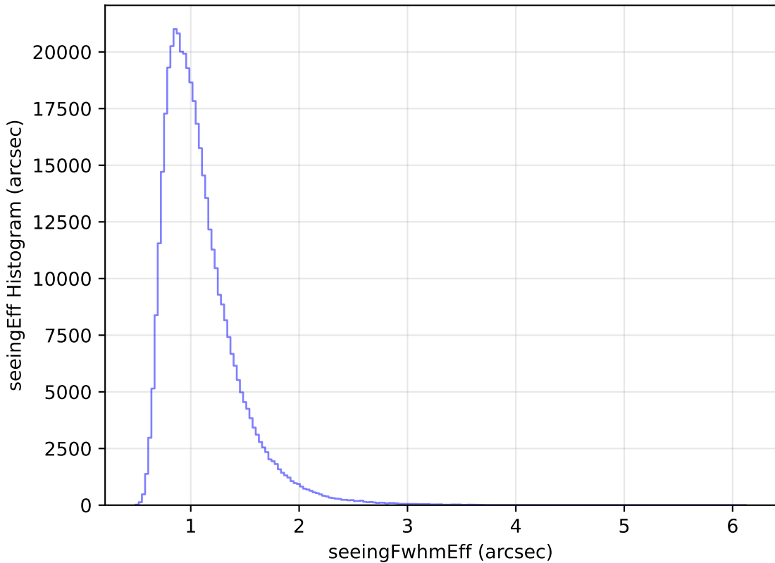
scp_reweight_v3.3_10yrs WFD z band: seeingEff Histogram
