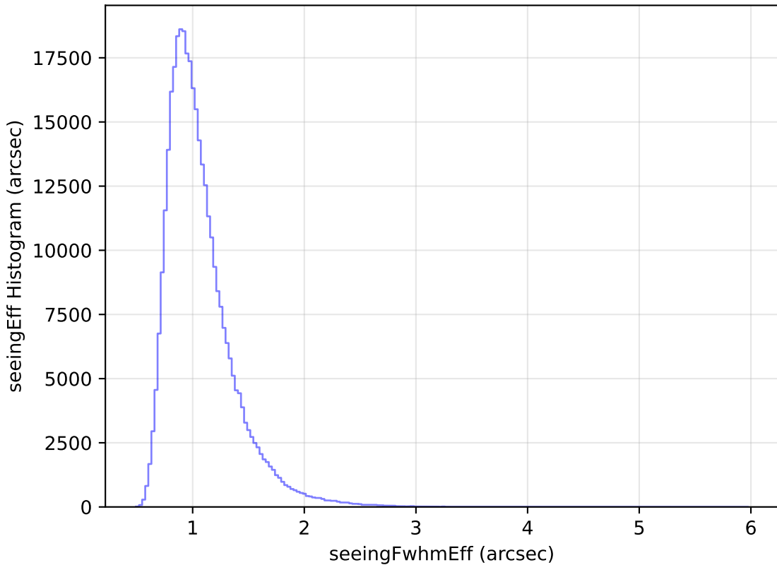
scp_reweight_v3.3_10yrs WFD y band: seeingEff Histogram
